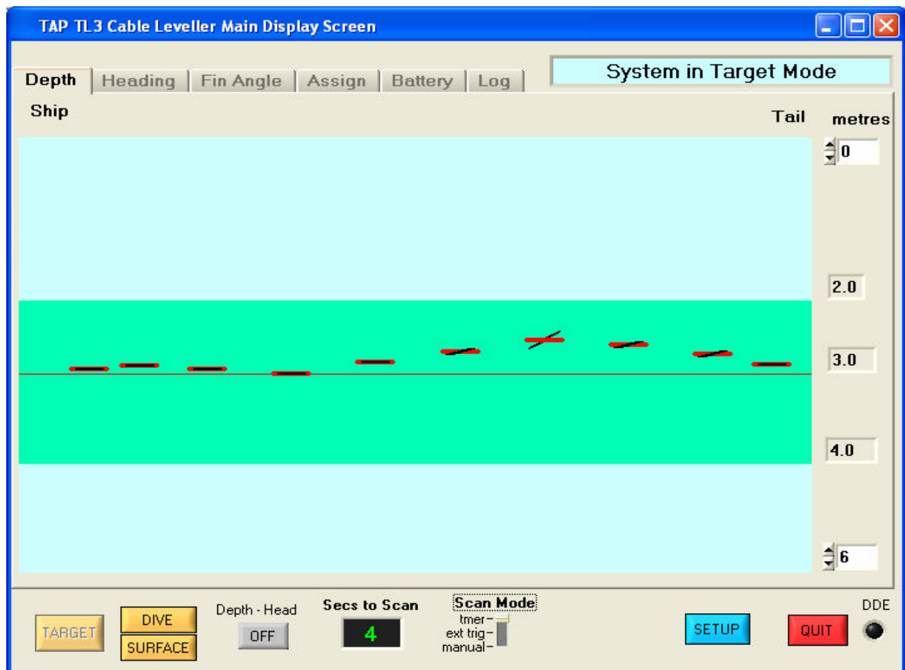
Depth Display Screen (simulated data)
